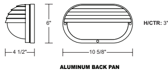
ALUMINUM BACK PAN
