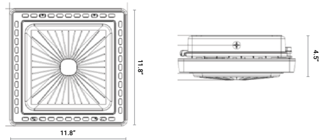
Model PGC100-100W
