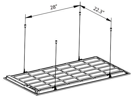
7502 4-Cable Kit
