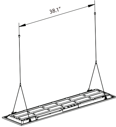
7501 2-Cable Kit
