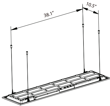
7502 4-Cable Kit
