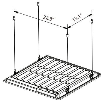
7502 4-Cable Kit
